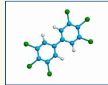
PCB molecule
